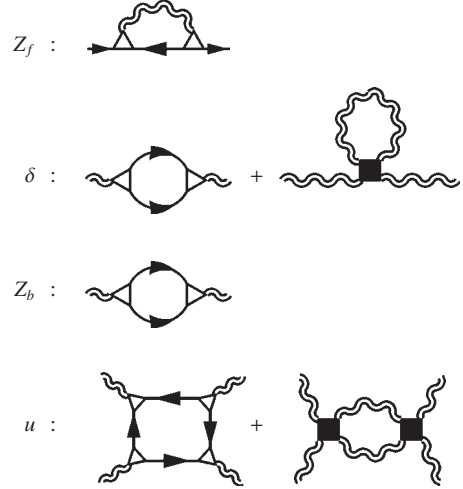
FIG. 4. Feynman diagrams representing the flow equations.
