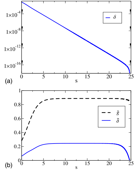
FIG. 6. (Color online) (a) Flow of the control parameter \delta at the QCP. (b) Flows of the rescaled control parameter and fermion-boson vertex as a function of s=-\ln[\Lambda/\Lambda_0] . The ultraviolet (infrared) regime is on the left (right) side of the plots.
