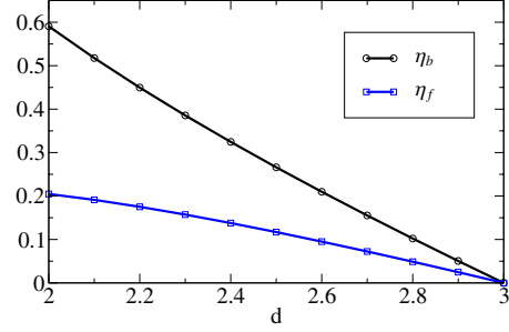
FIG. 5. (Color online) Fermion and boson anomalous exponents at the QCP for 2 \leq d \leq 3 .
