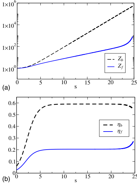
FIG. 7. (Color online) (a) Flows of the bosonic and fermionic frequency and momentum factors Z_b and Z_f . (b) Scaling plateaus of the fermion and boson anomalous dimensions at quantum criticality.
