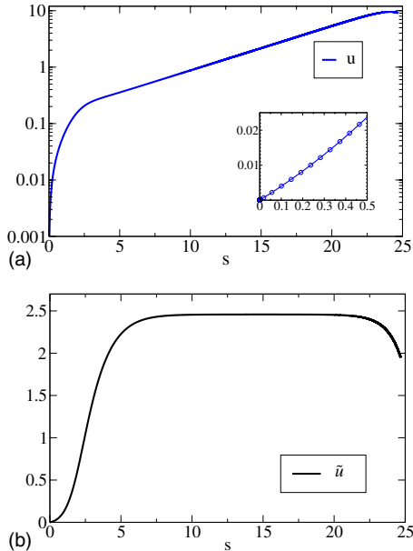
FIG. 8. (Color online) (a) Flow of the quartic coupling u . Inset: small- s behavior where fermionic fluctuations start generating u . (b) Fixed-point plateau of the rescaled \phi^4 coupling.
