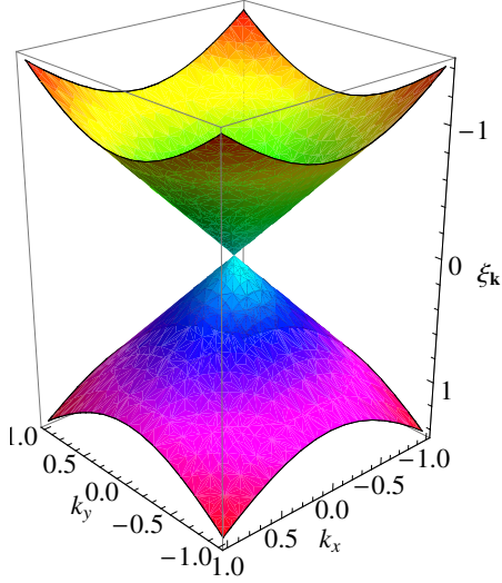
FIG. 2. (Color online) Dirac cone dispersion in two dimensions.
