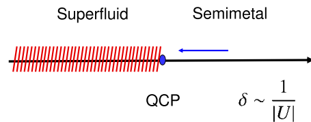
FIG. 1. (Color online) Schematic phase diagram of the attractive Dirac cone model at zero temperature. The QCP at a critical interaction strength U_c separates the semimetal from the superfluid. In this paper, we approach the QCP from the semimetallic phase as indicated by the arrow.
